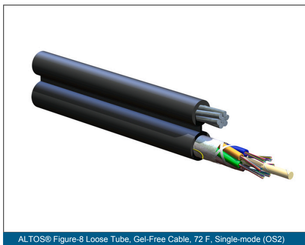
ALTOS® Figure-8 Loose Tube, Gel-Free Cable, 72 F, Single-mode (OS2)
