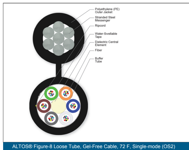
ALTOS® Figure-8 Loose Tube, Gel-Free Cable, 72 F, Single-mode (OS2)
